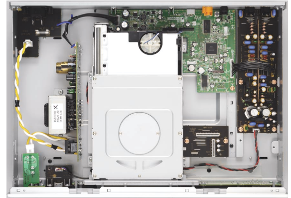
CD-S700 Interior view with silent loader and high precision CD drive
