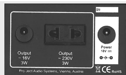
Rear panel: DC in & AC out
