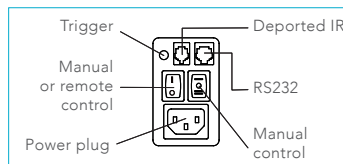
Remote control
